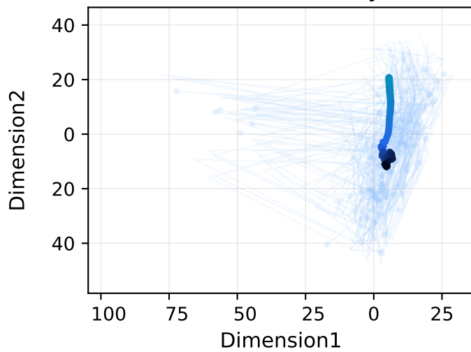
Self-consistency
