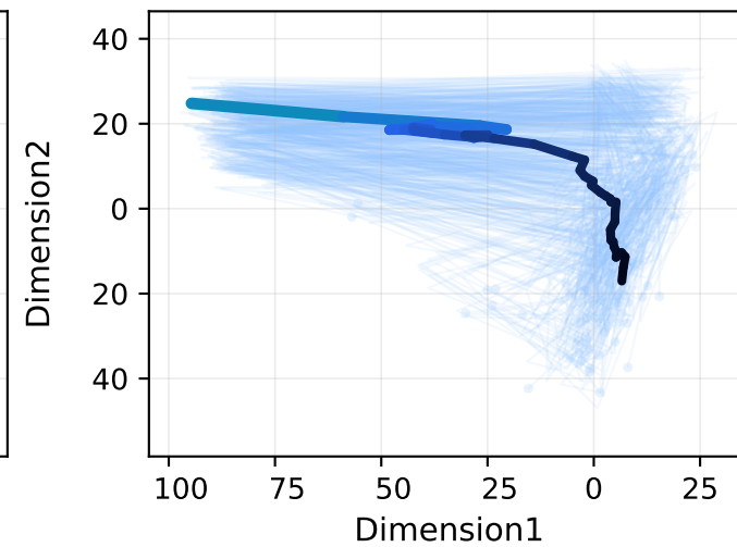
Constrained beam
