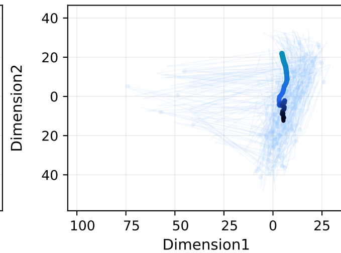
Best-of- N
