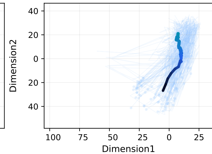
MCTS
